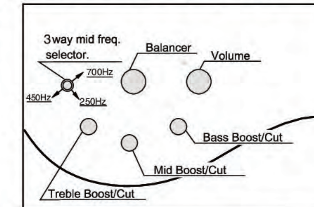
BEQIII 3band-EQ w/3way mid freq. selector
