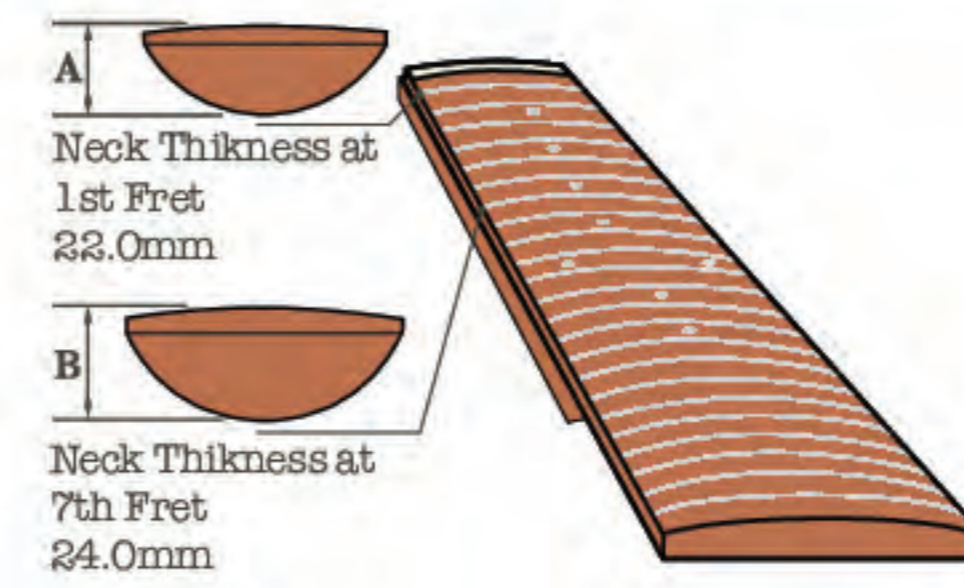
Neck Dimension
