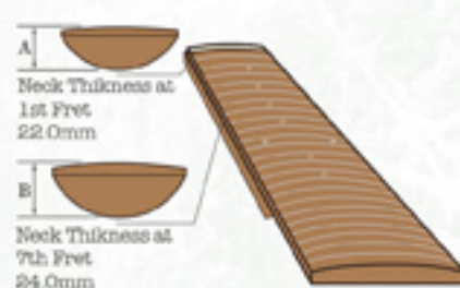
Neck Dimension
