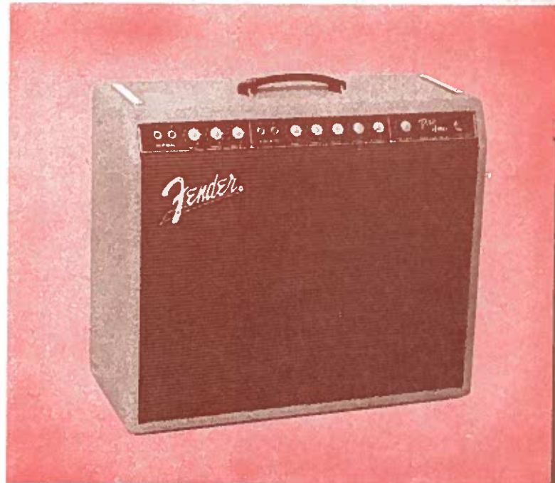
PRO AMP —Tubes: 1—Silicon Rectifier, 2—6L6GC, 5—7025 (each dual purpose). Speakers: 1—15" Heavy Duty Jensen Concert Series. Size: Height, 20"; Width, 24"; Depth, 10 1/4".
